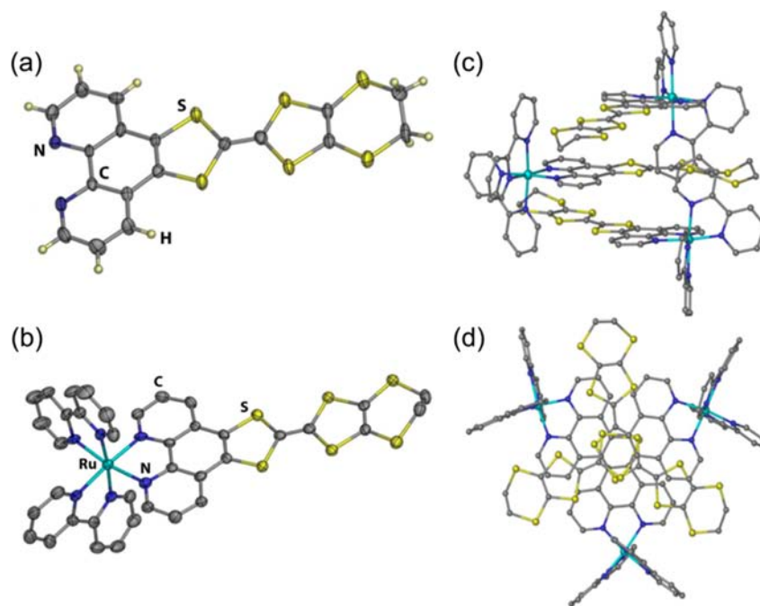
Figure 2. (a, b) Molecular structures of ligand L1 and its Ru(II) complex, [\text{Ru}(\text{bpy})_2(\text{L1})]^{2+} . Thermal ellipsoids are at the 50% probability level. (c, d) Side and top views of the packing of [\text{Ru}(\text{bpy})_2(\text{L1})]^{2+} cations in the crystal structure of 1 ·3.6 \text{CH}_3\text{CN} . In b–d, the H atoms have been omitted for clarity. Color scheme: Ru, light blue; S, yellow; N, blue; C, gray; H, off-white.
