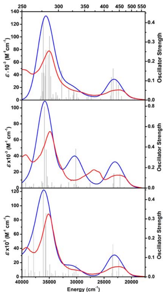
Figure 5. Experimental (red line) and simulated (blue line) optical absorption spectra of 1–3 (top to bottom, respectively). The gray bars indicate the energy and oscillator strength of each electronic excitation.
