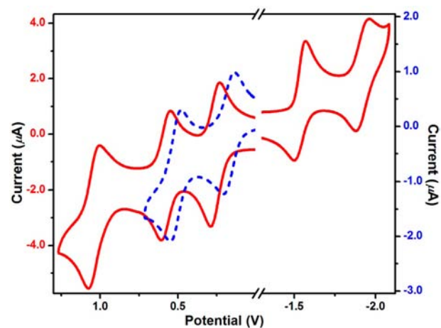
Figure 3. Cyclic voltammograms of L1 and 1 (dashed blue and solid red lines, respectively) recorded in a 0.100 M solution of (\text{Bu}_4\text{N})\text{PF}_6 in \text{CH}_3\text{CN}/\text{CH}_2\text{Cl}_2 (3:2 v/v) at 0.100 V/s. Potentials are given vs \text{Fc}/\text{Fc}^+ .
