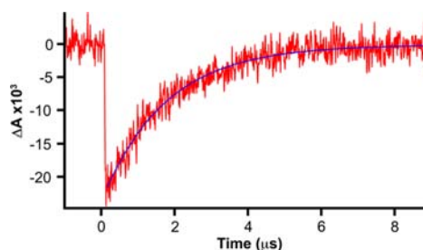
Figure 6. Kinetic profile of the difference absorbance spectrum of 1 in \text{CH}_3\text{CN} at room temperature. \lambda_{\text{pump}} = 488\text{ nm} ; \lambda_{\text{probe}} = 458\text{ nm} . Experimental data, red; single exponential fit, blue.
